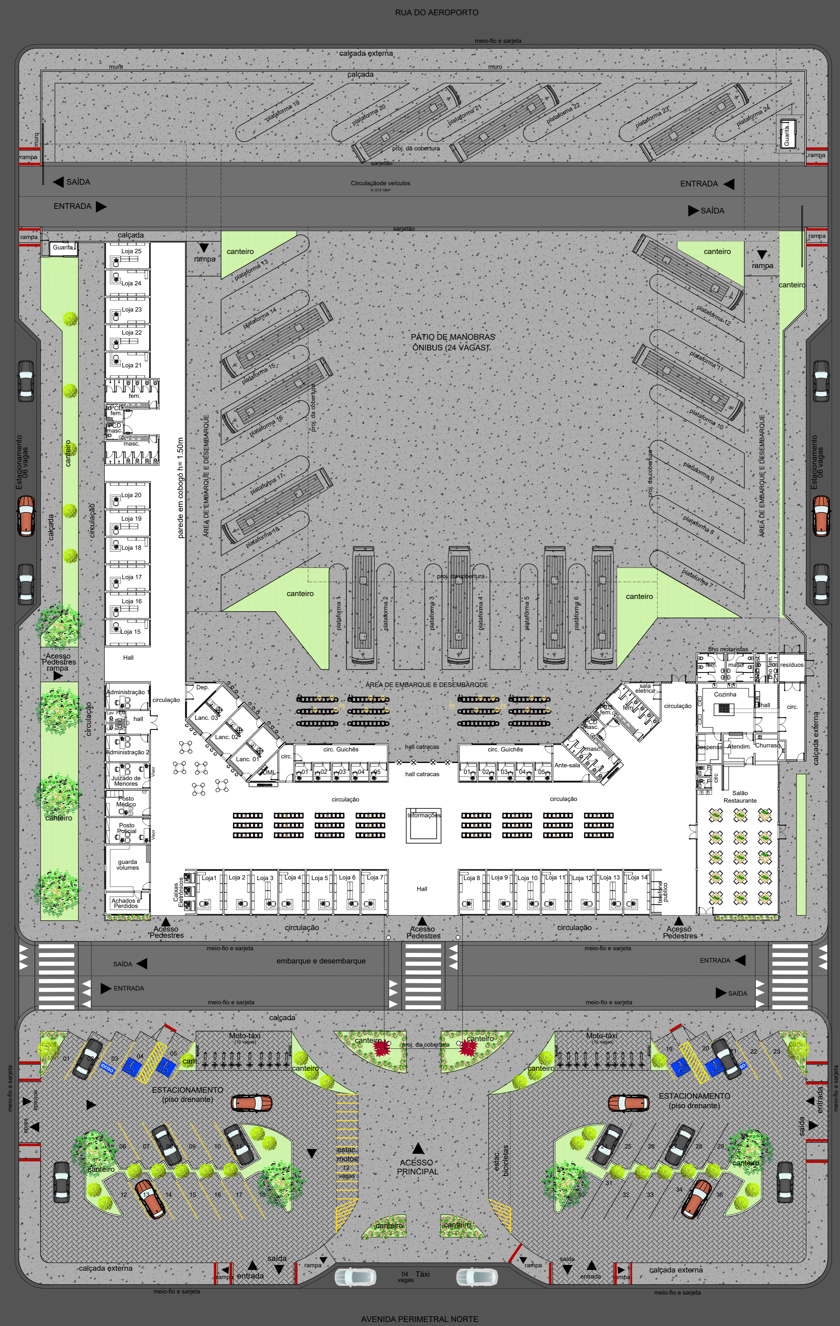
Layout Escala 1:250
